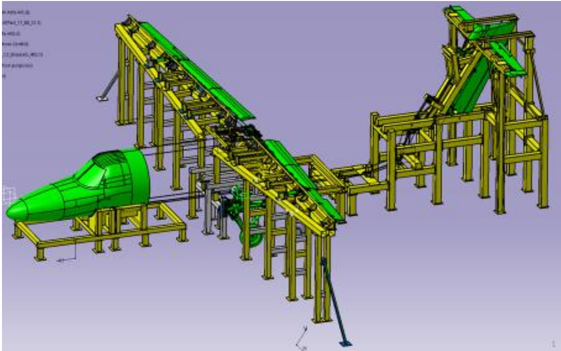
Figure 2. Iron Bird Structural Frame (indicative)
