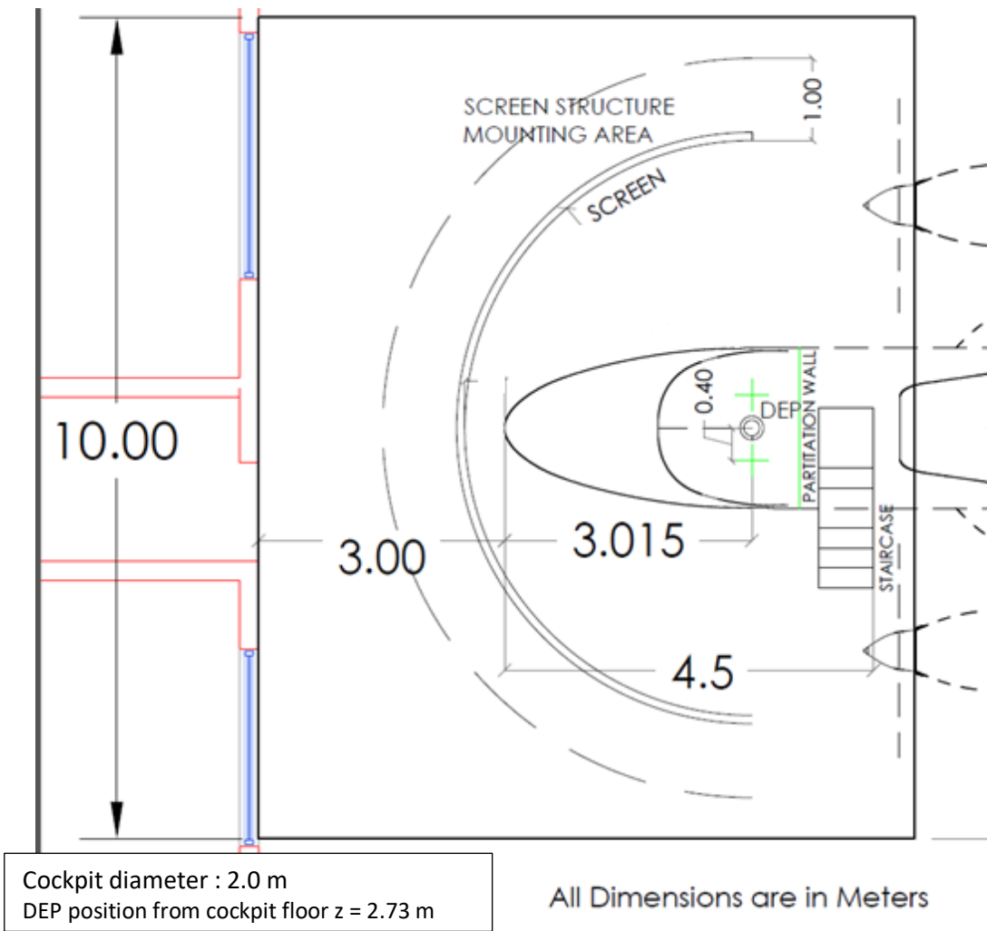
Figure 1b. Cockpit area expanded
