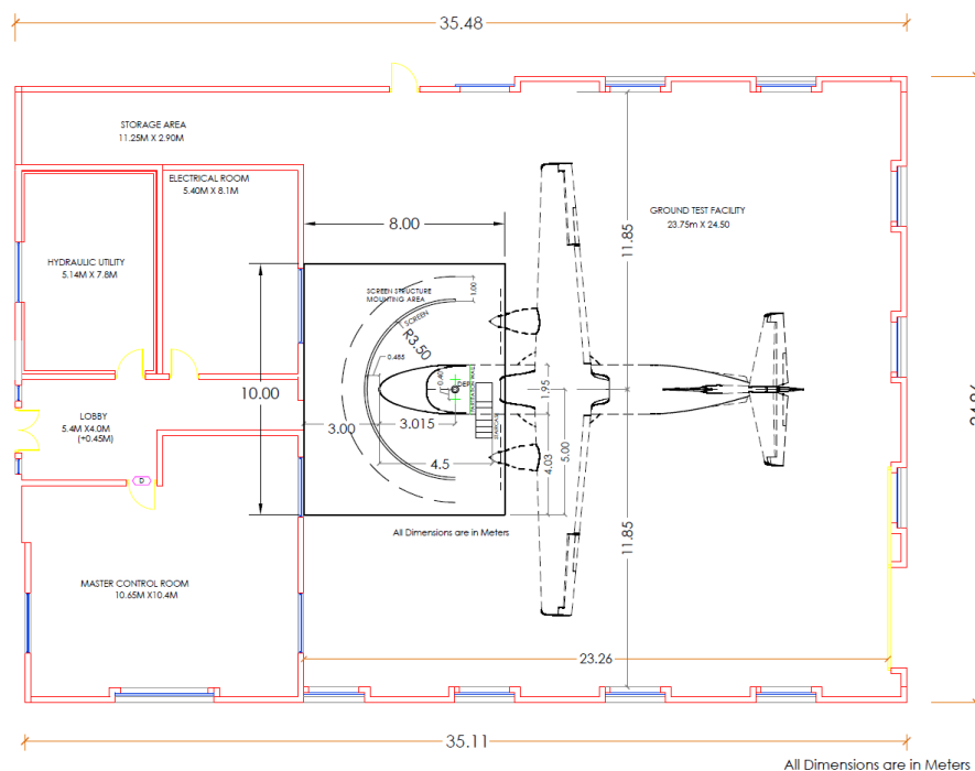
Figure 1a. Layout of the Iron Bird facility.
