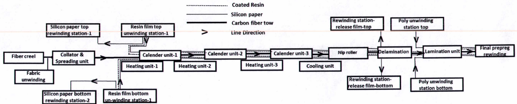
Schematic diagram of carbon fiber prepreg line
