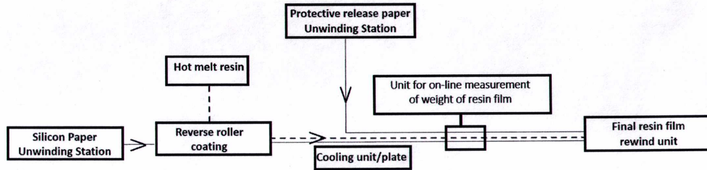
Schematic diagram of hot melt resin coating machine
