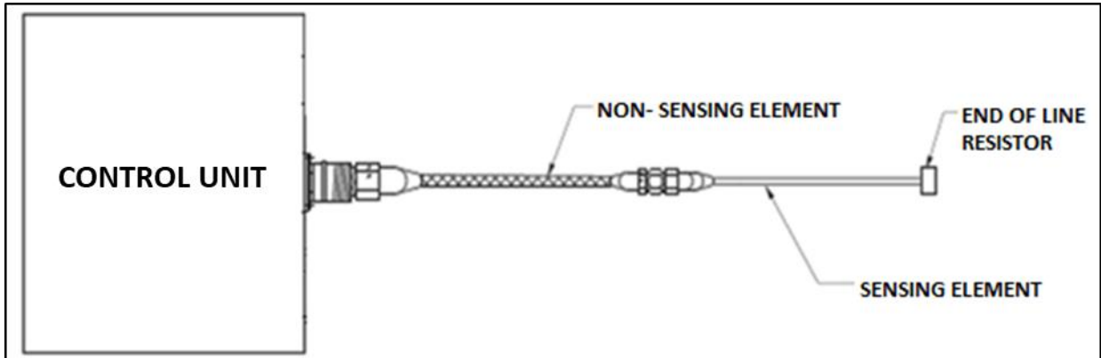
Figure 1: Schematic Diagram of BALD System (LH / RH Wing) (Typical)
