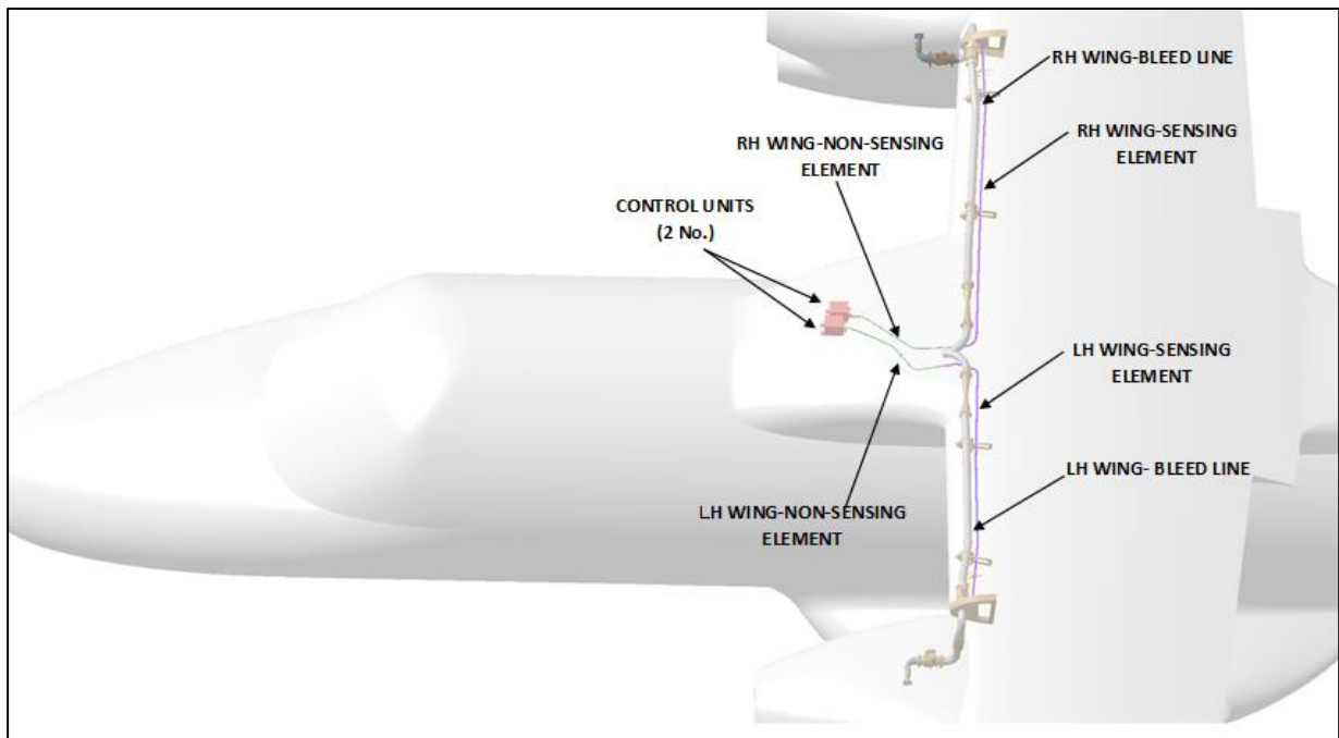
Figure 2: BALD System Implementation Layout (Typical)
