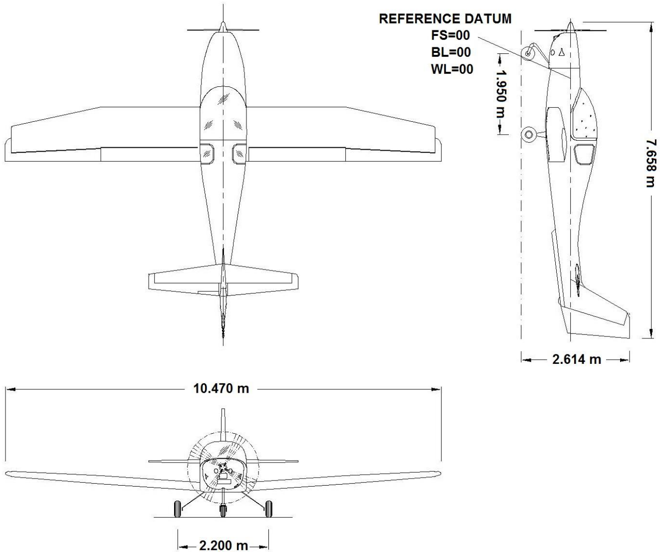
Figure 1: Fig. 1: HANSA-3 three view drawing
