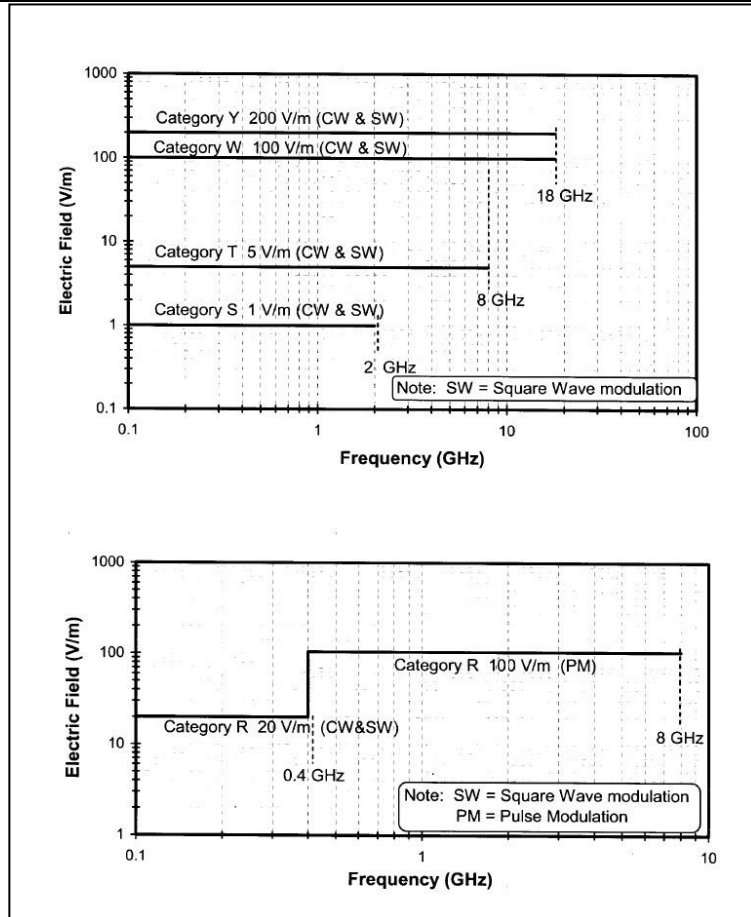
Modified Figure 20-10 (A&B) Radiated Susceptibility Test Level for SARAS Mk II Aircraft
