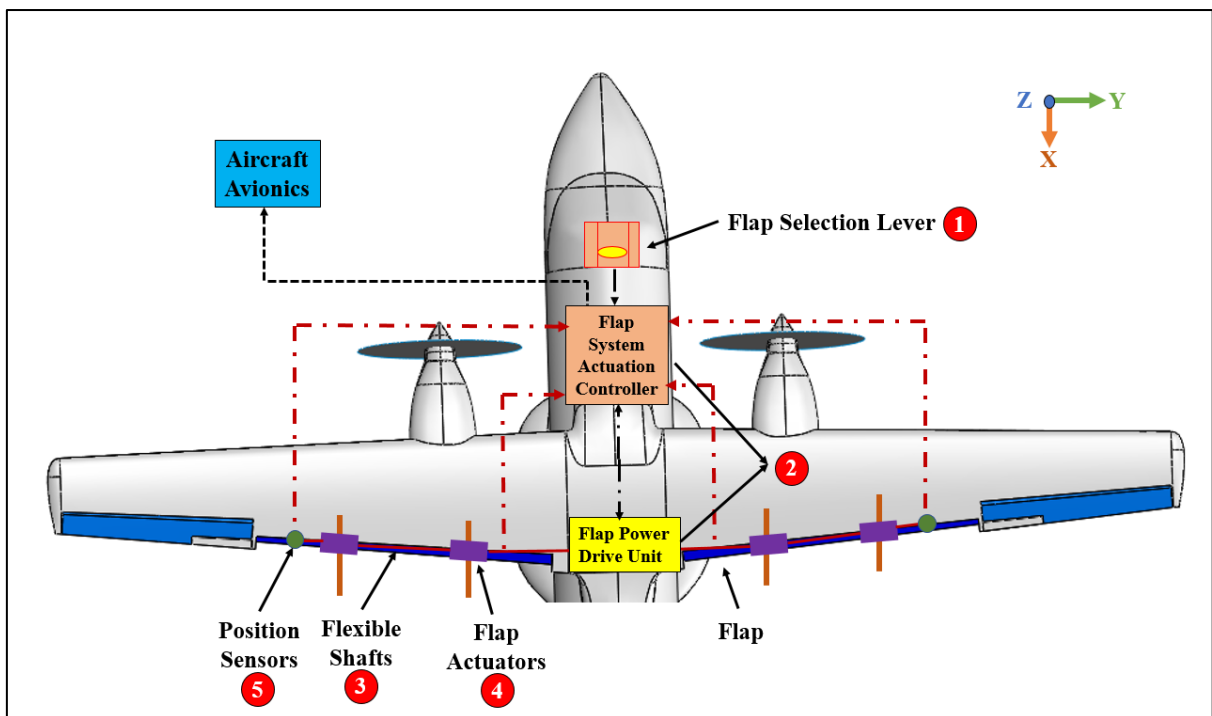
Figure 1 Typical schematic of Flap Control System
