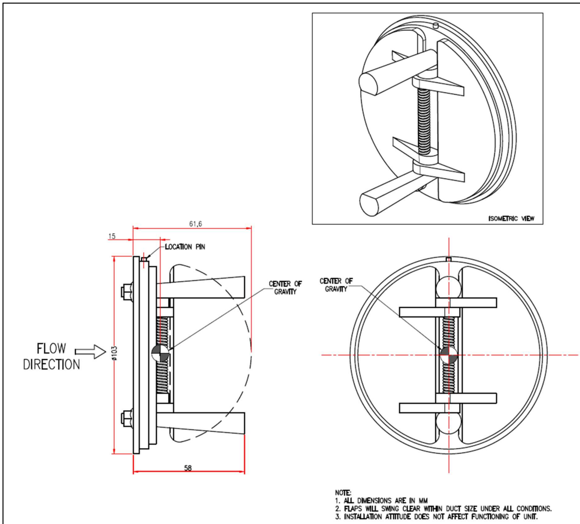
Figure 1: 4-inch NRV Schematic
