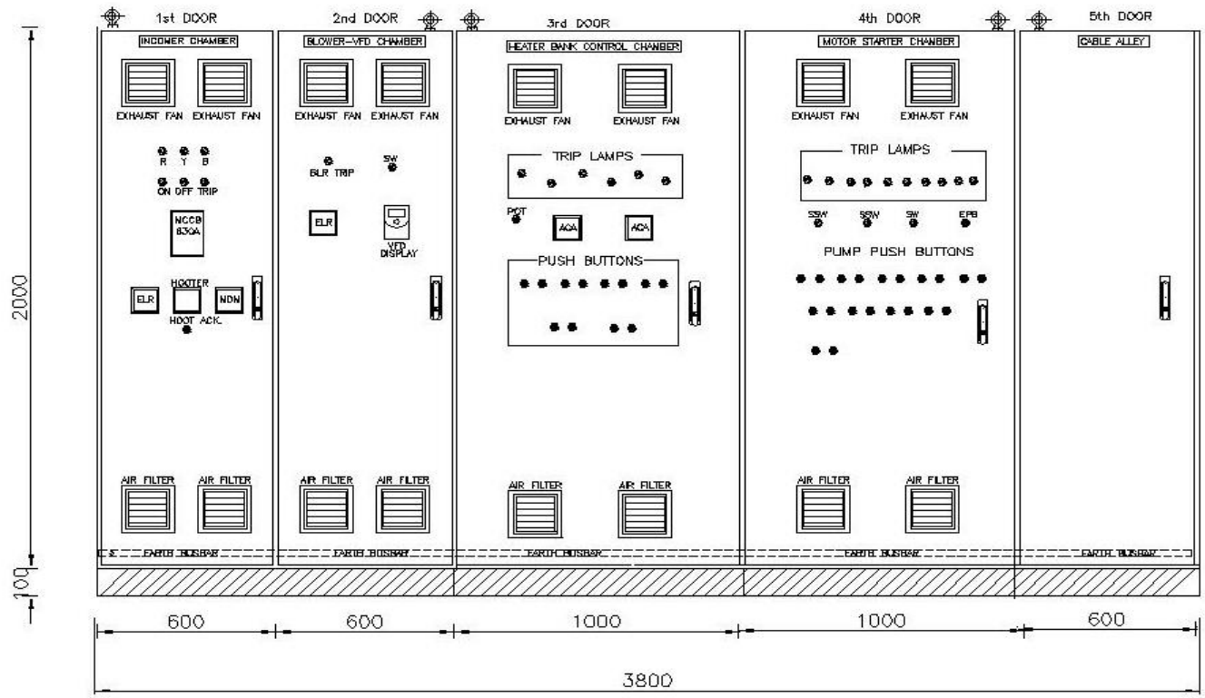
FRONT VIEW
