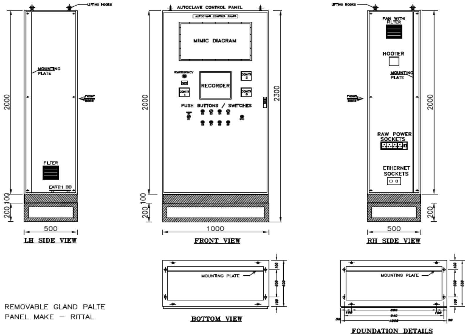
Fig 3: Control Panel General Arrangement drawing
