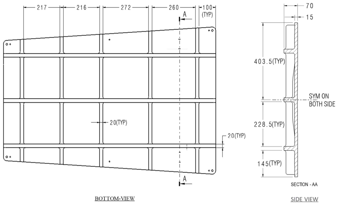
Figure 8: Tool for Wing-Fuselage Center Fairing Aft Side (LH & RH) (Side View and Bottom View)
