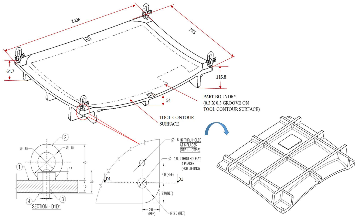
Figure 1: Tool for Wing-Fuselage Front Fairing Mid Center Skin
