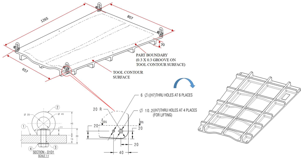
Figure 7: Tool for Wing-Fuselage Center Fairing Aft Side (LH & RH)
