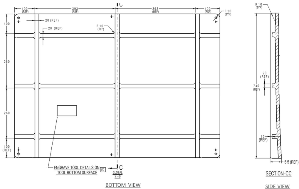
Figure 4: Tool For Wing-Fuselage Front Fairing Mid AFT SKIN (Side View and Bottom View)
