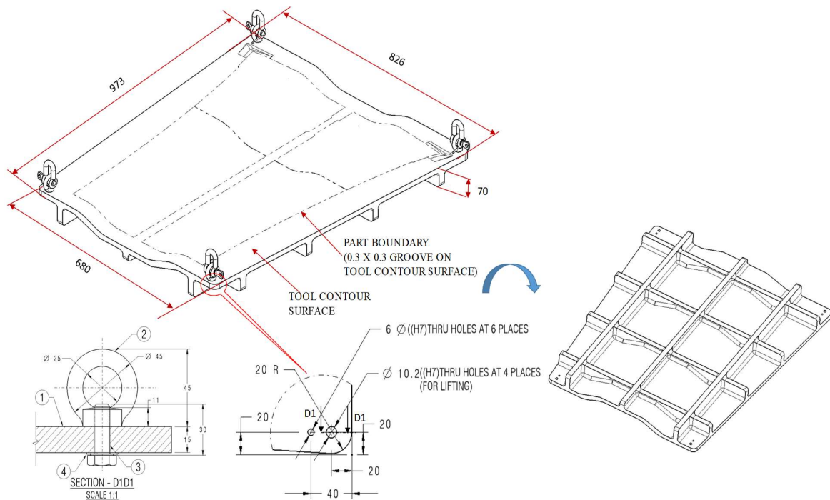
Figure 5: Tool for Wing-Fuselage Center Fairing Fwd Side (LH & RH)
