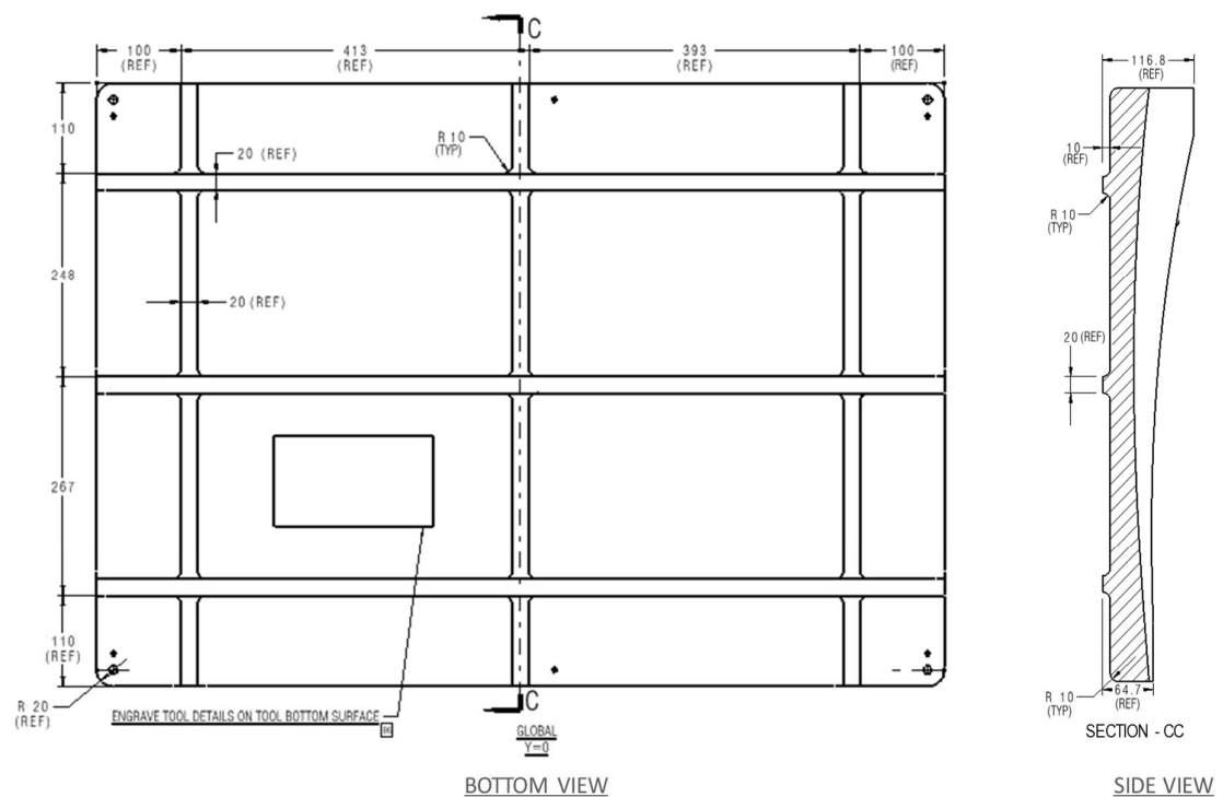
Figure 2: Tool for Wing-Fuselage Front Fairing Mid Center Skin (Side View and Bottom View)
