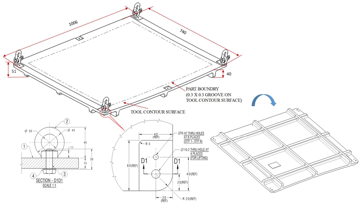
Figure 3: Tool for Wing-Fuselage Front Fairing Mid AFT SKIN
