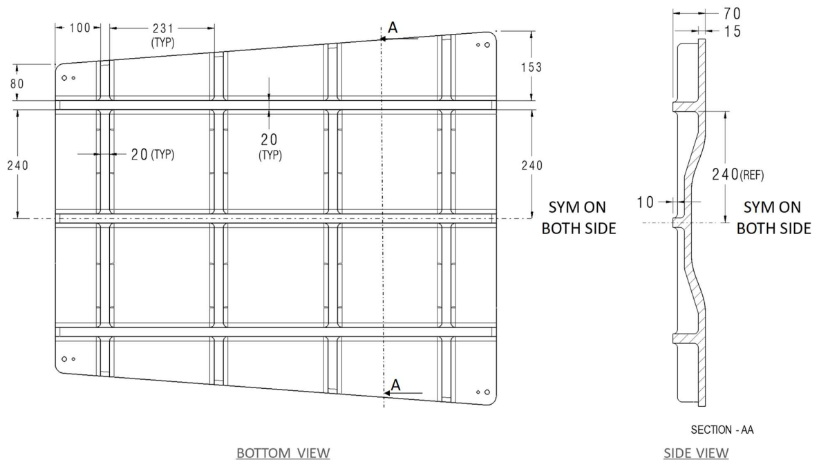
Figure 6: Tool for Wing-Fuselage Center Fairing Fwd Side (LH & RH) (Side View and Bottom View)
