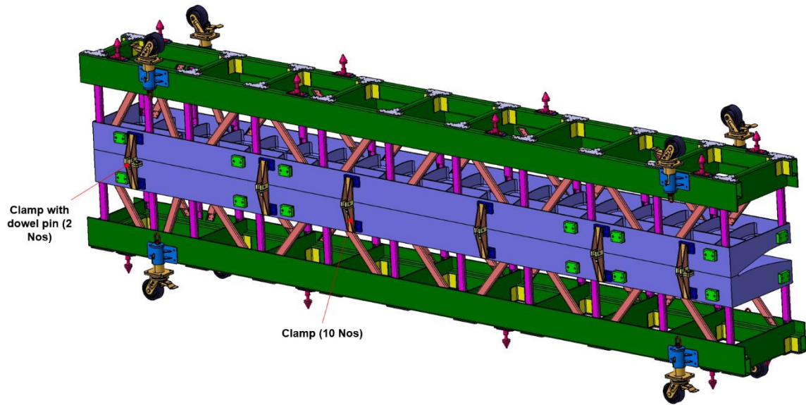
Figure 6. Bottom & Top moulds are in assembled condition
