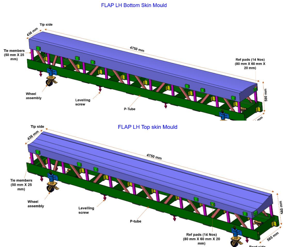
Figure 5. Overall Dimension of the Flap LH Mould (Top)
