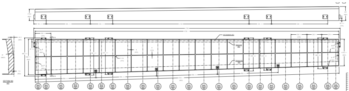
Figure 7. Flap Aft Box mould (LH) plan view with dimensions
