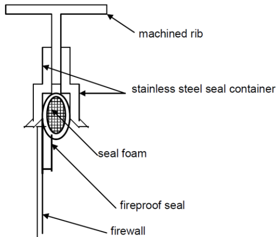
Fig. 5: Firewall seal typical cross section.
