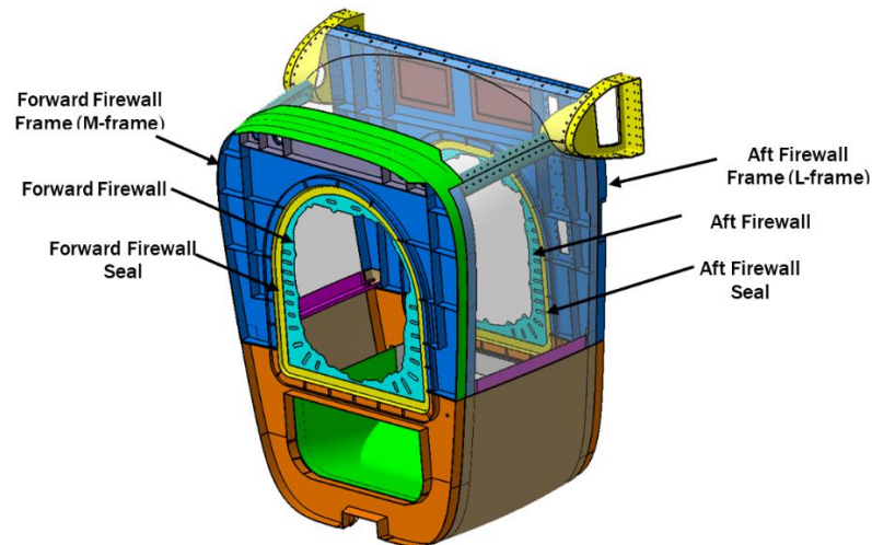
Figure 3: Centre nacelle assembly (w/o engine and mounts)
