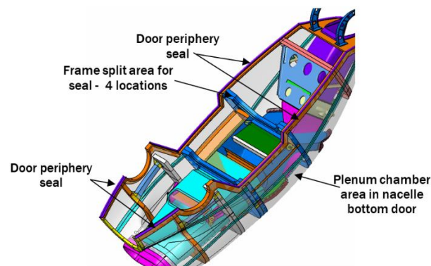
Figure 4: Hinged nacelle door with seal requirement.
