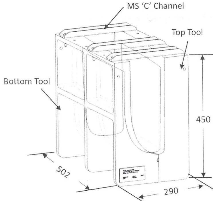
Figure 1: Wing tip skin tool
