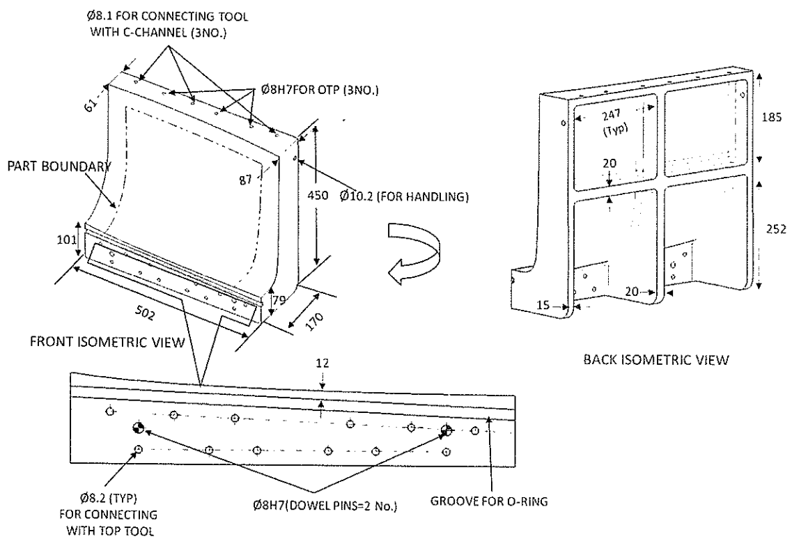
Figure 3: Bottom skin tool
