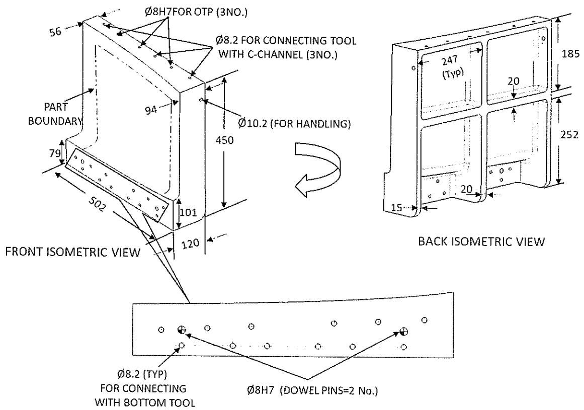
Figure 2: Top skin tool
