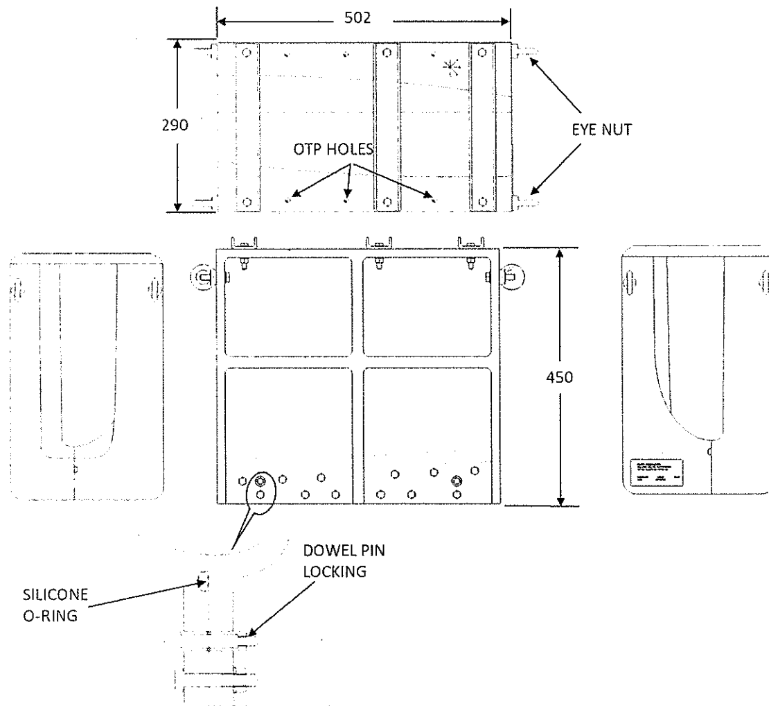
Figure 3: Assembly of top and bottom tools
