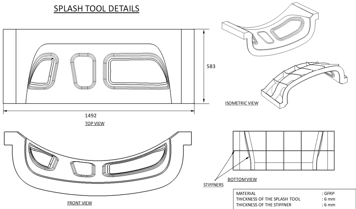
Figure 9. Orthographic and Isometric view of splash tool for Wing-Fuselage Front Fairing Mid Side Skin (LH & RH)
