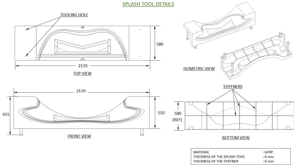
Figure 13. Orthographic and Isometric view of splash tool for BLISTER FAIRING BAY-07(#22-#23)
