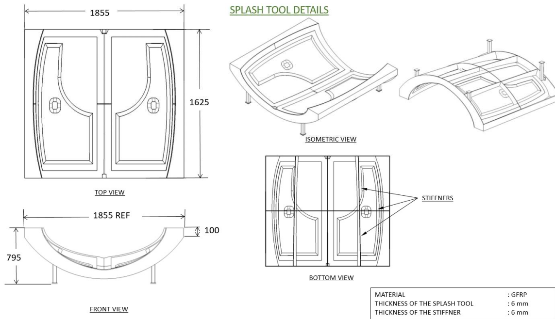
Figure 11. Orthographic and Isometric view of splash tool for BLISTER FAIRING AT BAY-4 DOOR #17-#20 (LH&RH)
