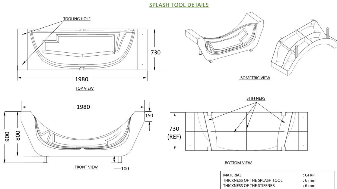
Figure 9. Orthographic and Isometric view of splash tool for BLISTER FAIRING AT BAY_01 (#13-#14)
