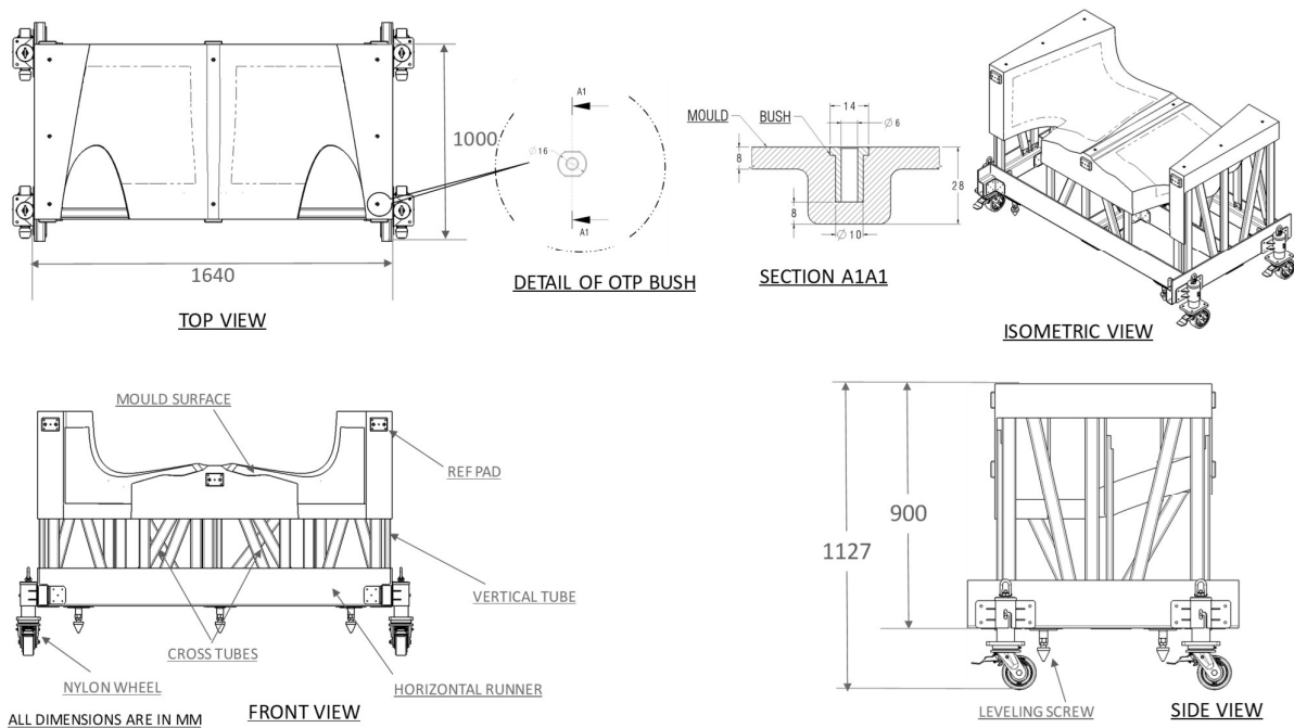
Figure 7. Orthographic and Isometric view of tool for Wing-Fuselage front fairing aft side skin (LH & RH)
