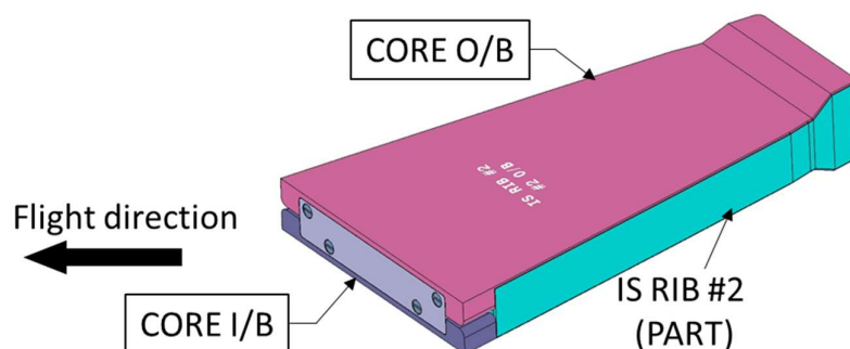
Assembly of IS Rib Core I/B & O/B
