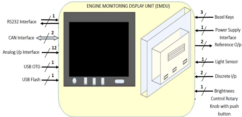
Figure 1: System Level Interface Block Diagram of EMDU
