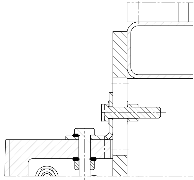
SECTION N1-N1
