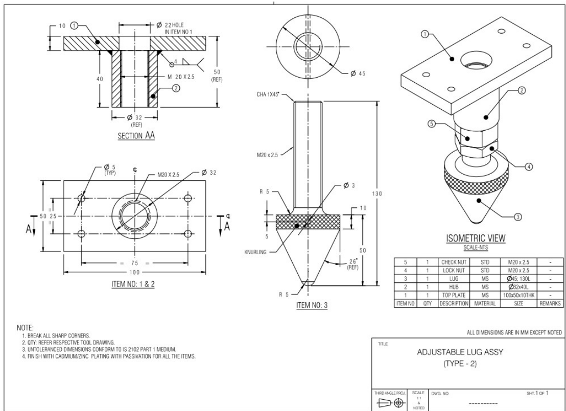
(Item 1, g) Adjustable Lug Assembly for Item (1)
