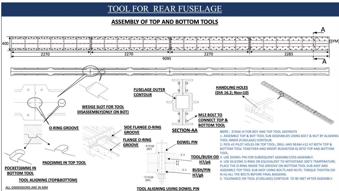
(Item 1.d ) Top/Bottom Tool Assembly
