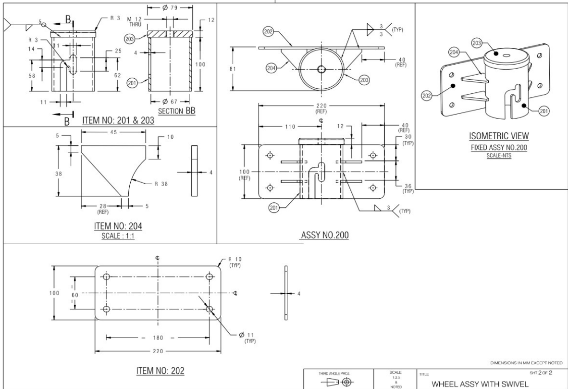
(Item 1, g) Wheel Assembly for Item (1)
