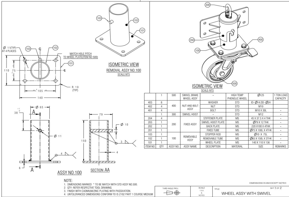
(Item 1, f) Wheel Assembly for Item (1)
